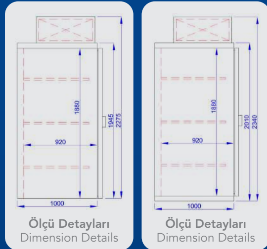
CN100-WF Tabansız Without Floor
