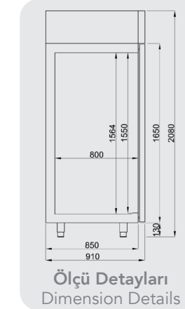
48 adet 17x36x12 Dondurma Kabı Kapasiteli 48 units 48x36x12 Ice Cream Cup Capacity
